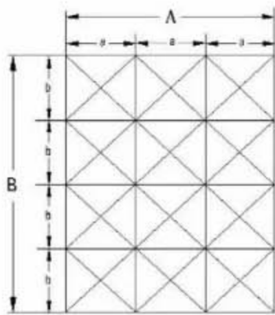
图 2 矩形风口测点布置
